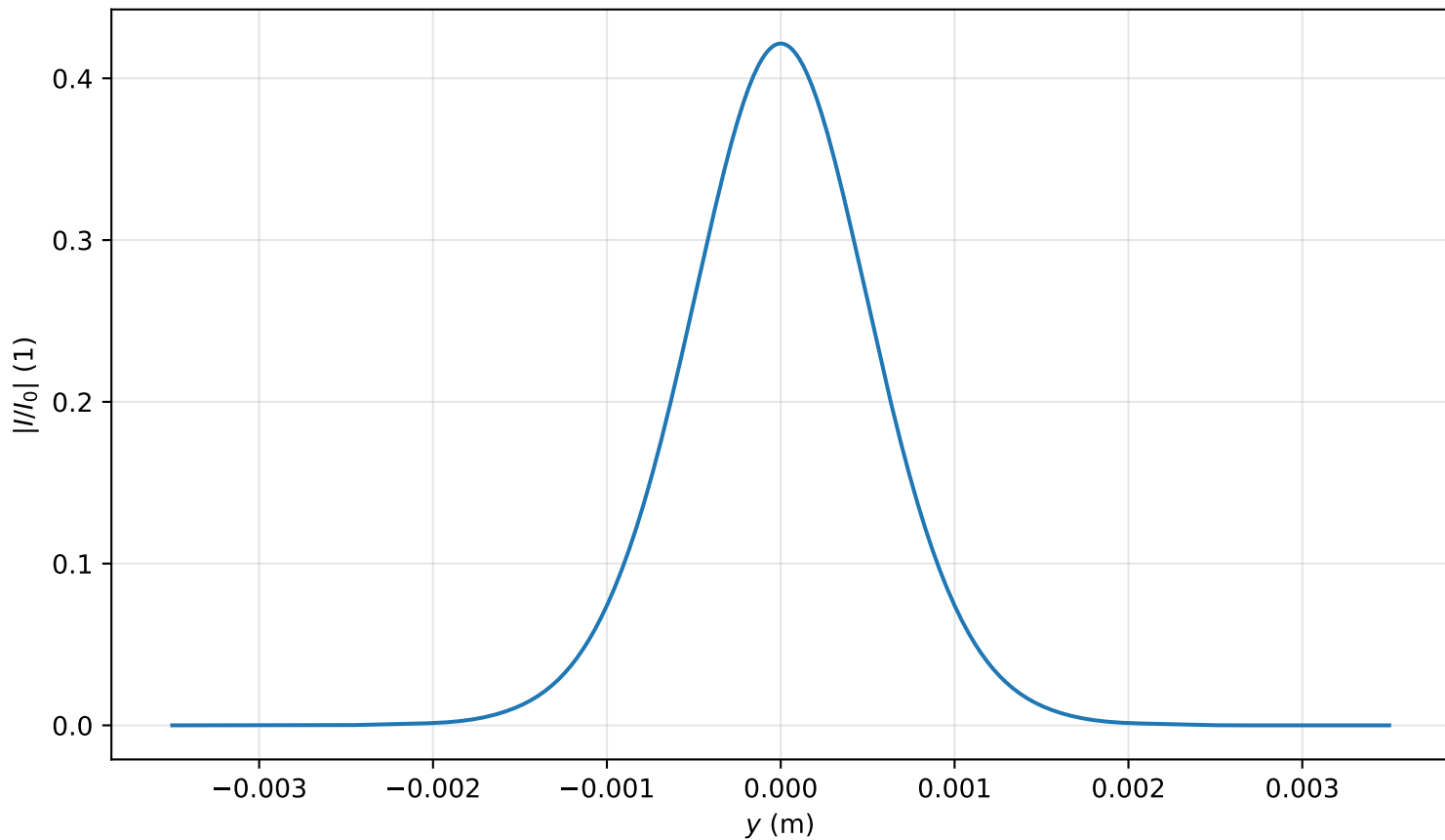
Intensity profile I(x=0, y, z=3.344)/I_0 , P_{in}=0.4P_{cr} , artificial time
